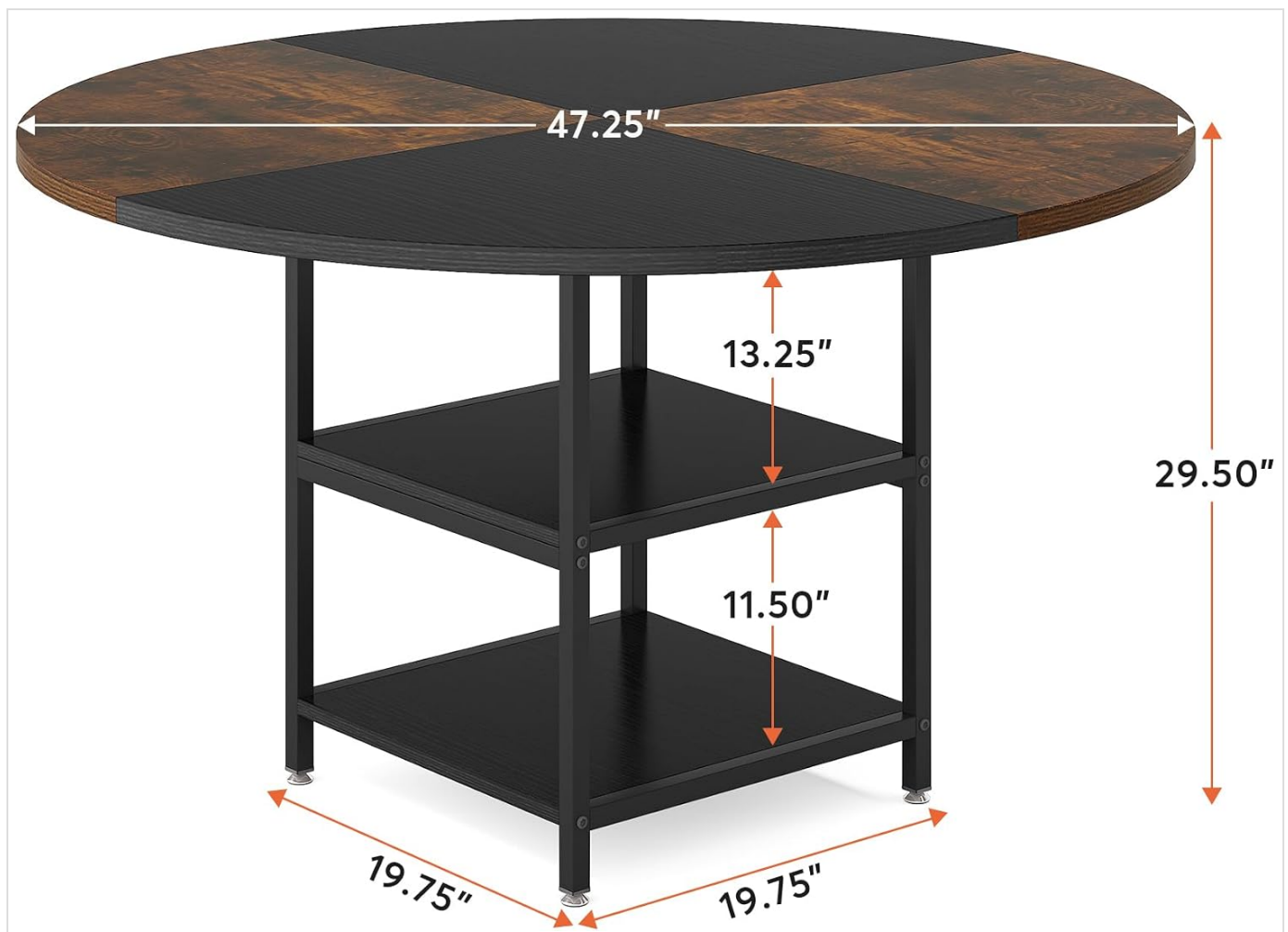
Image: Detailed dimensions of the dining table, including height, width, and shelf clearances.
