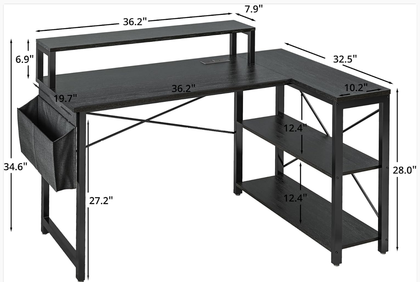
Image 3.1: Diagram illustrating the key dimensions of the IRONCK L Shaped Desk, including the main desktop, L-extension, monitor stand, and storage shelves.
