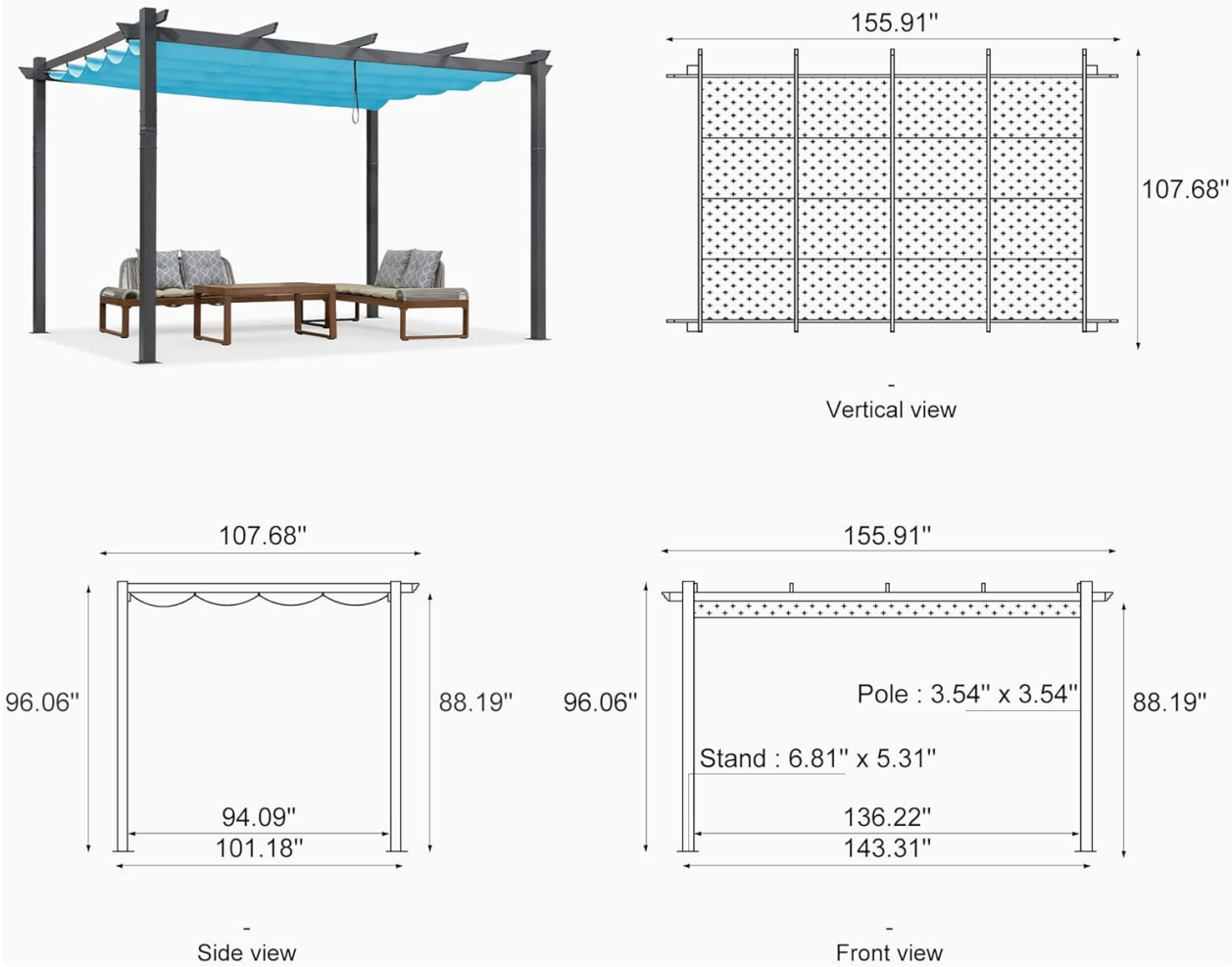
Figure 8: Detailed product dimensions.
