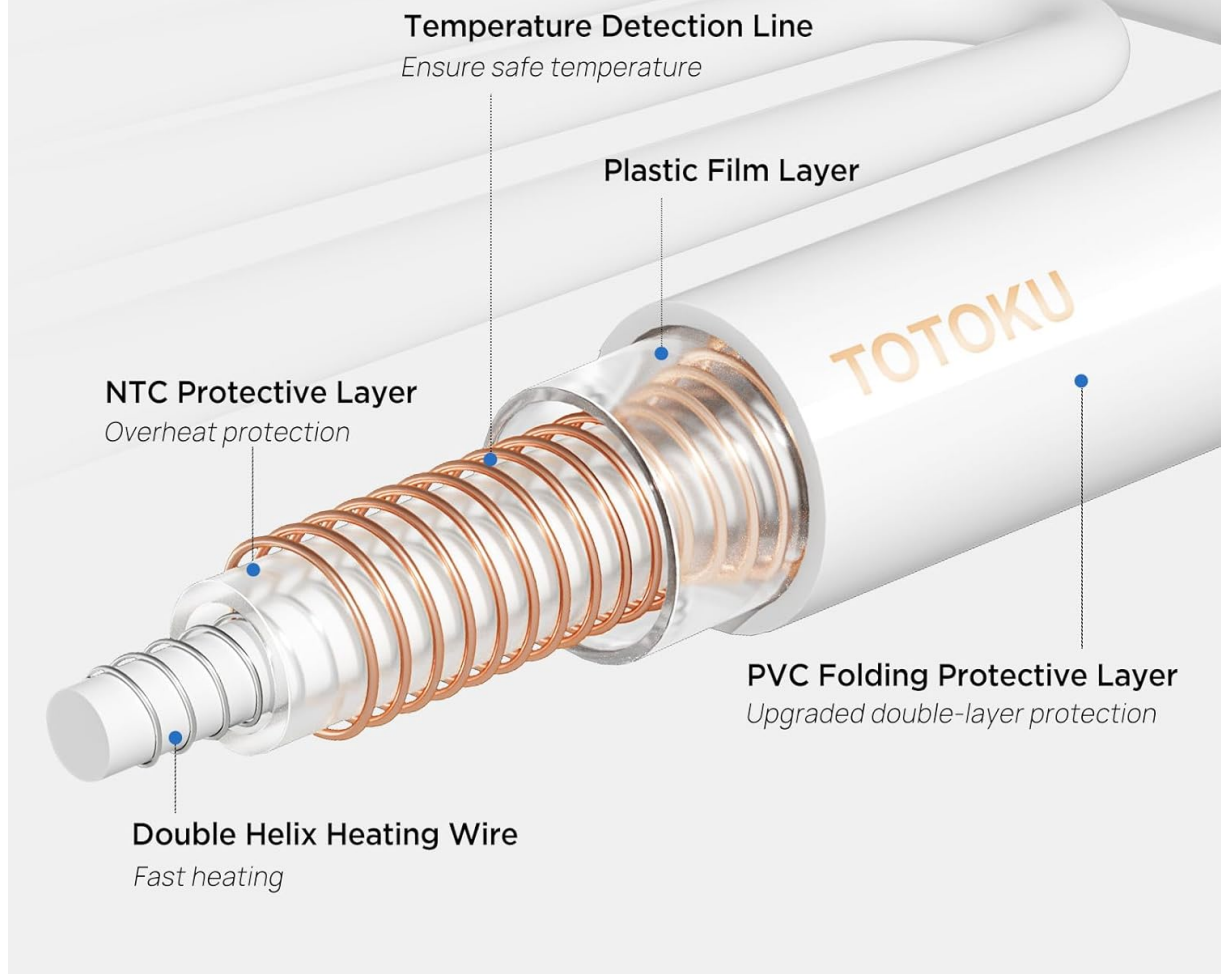
Image: Internal safety wiring diagram.
