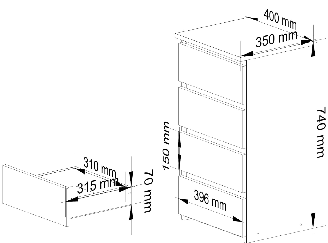
Figure 1: Product dimensions and drawer component measurements for assembly reference.
