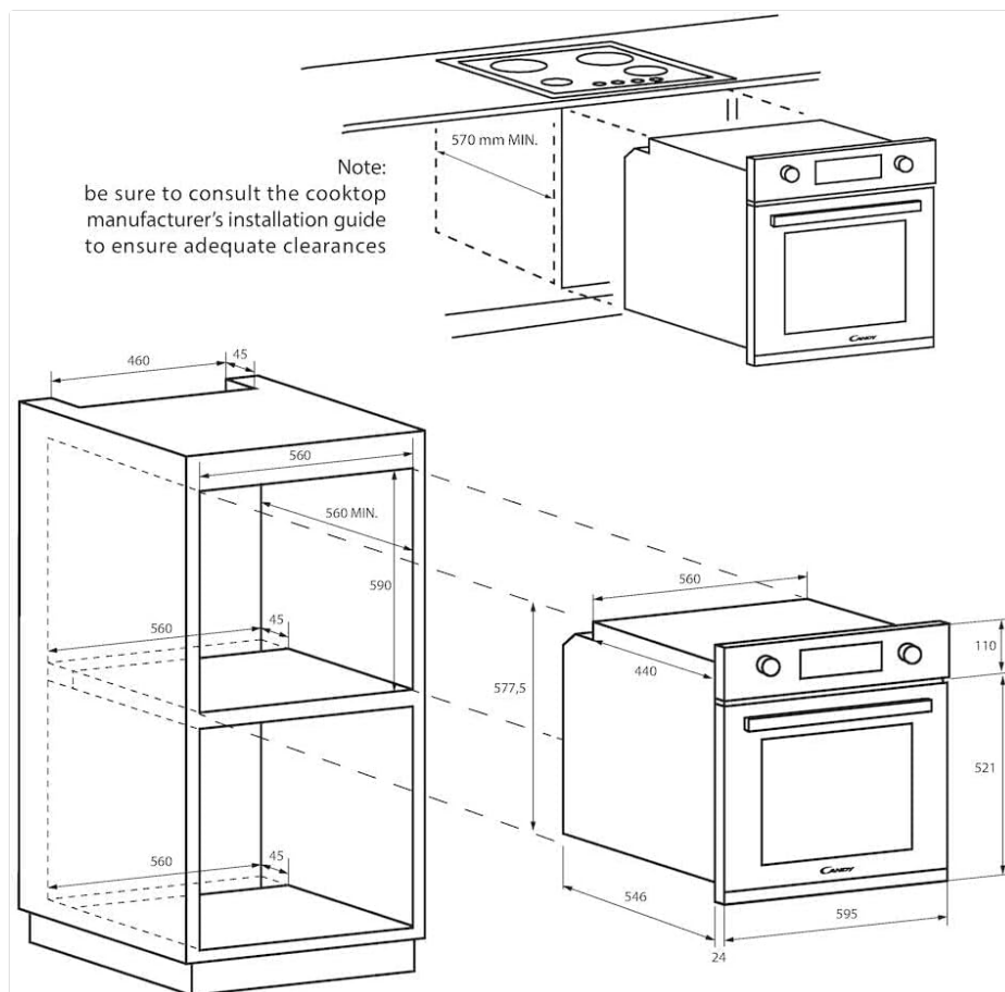
Figure 4.1: Detailed technical diagram illustrating the oven's dimensions and the required integration niche measurements for proper installation. Consult the cooktop manufacturer's installation guide for adequate clearances.
