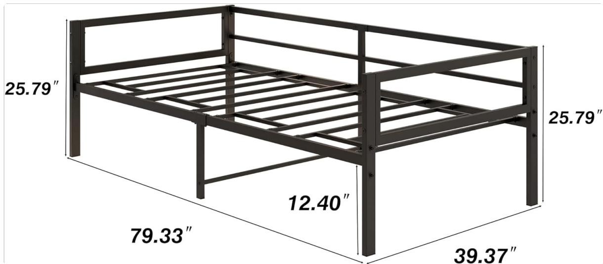
Image: A technical diagram illustrating the key dimensions of the DUMEE Twin Day Bed Frame, including length (79.33"), width (39.37"), height (25.79"), and under-bed clearance (12.40").
