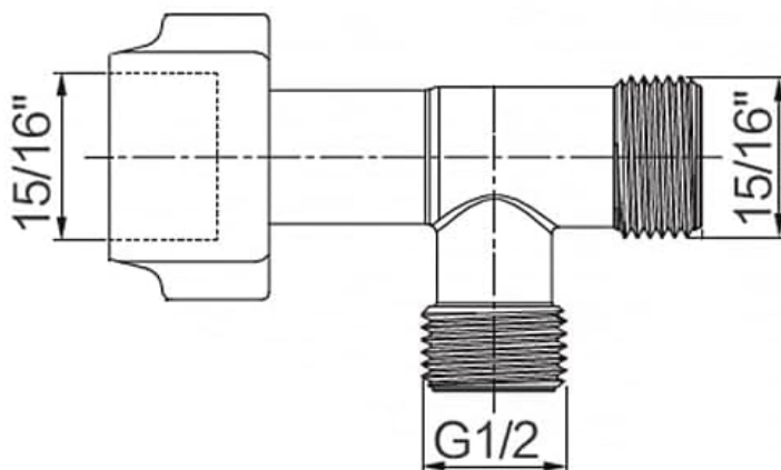
Figure 6: T-valve dimensions and connection specifications.
