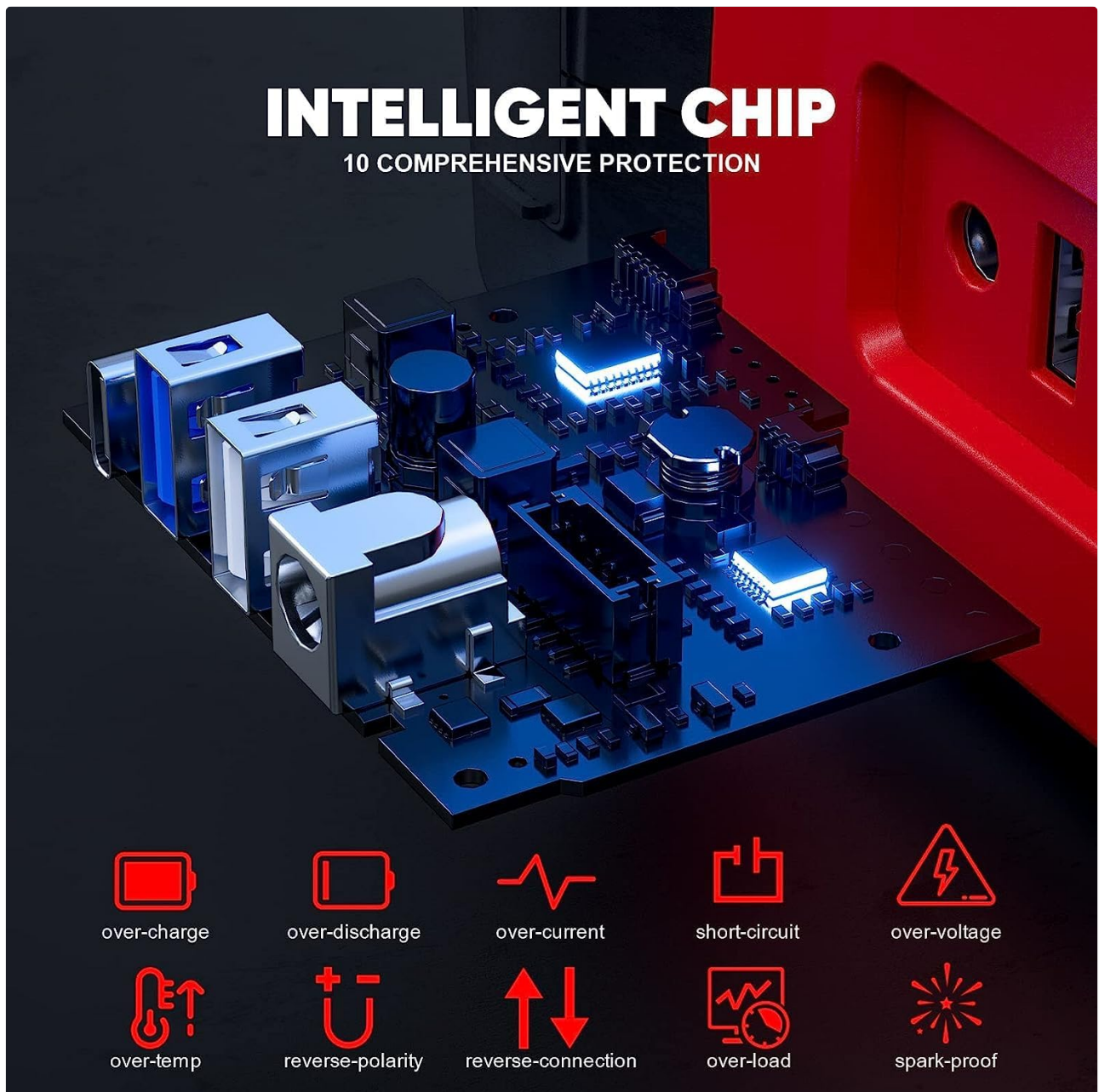
Figure 5: The intelligent chip provides comprehensive safety protection.
