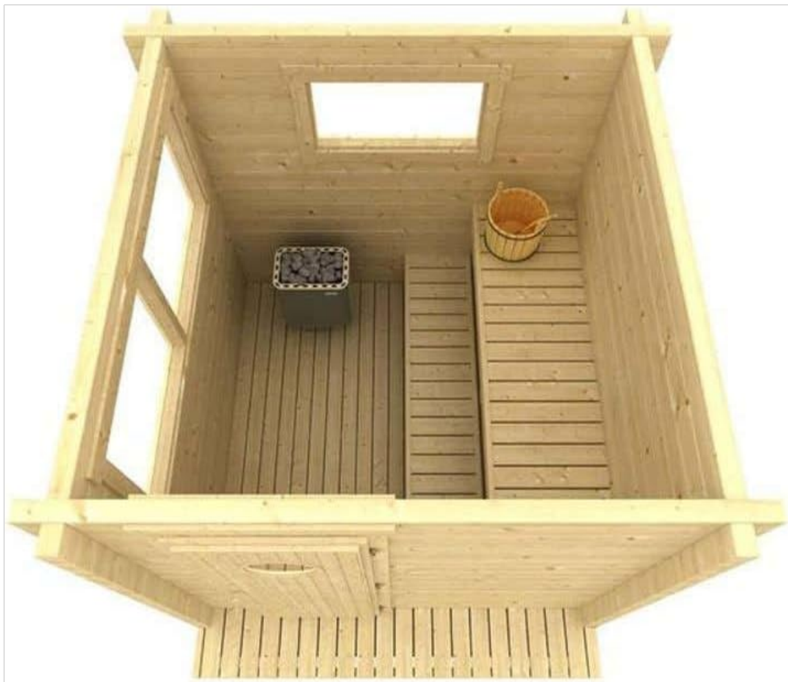
Figure 2: Top-down structural view of the sauna, detailing the interior layout and component placement.
