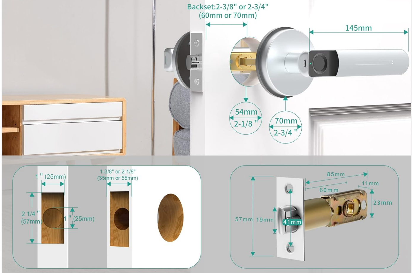
Image: Door dimensions and latch backset measurements for proper installation.
