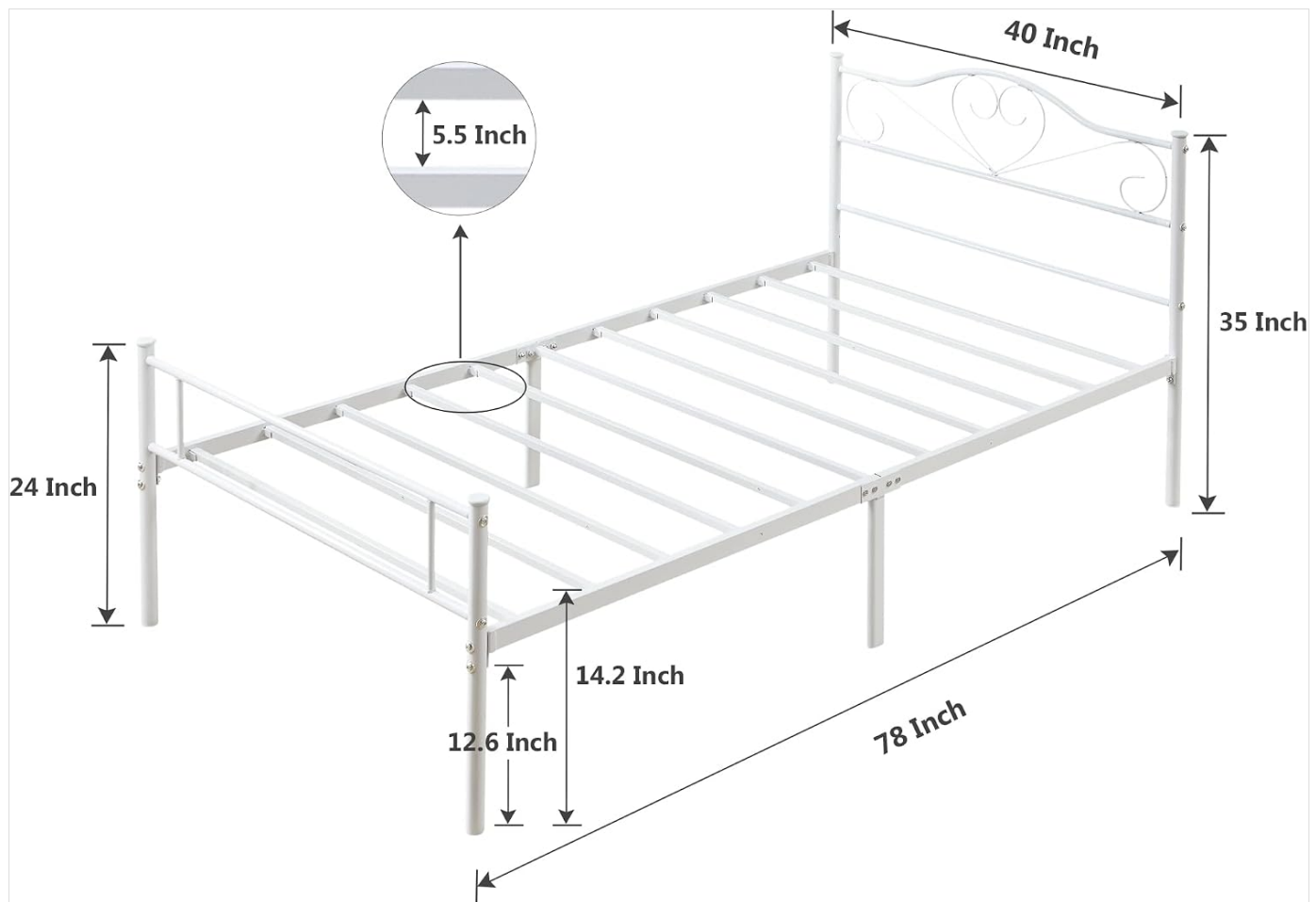
Image: A detailed diagram illustrating the key dimensions of the VECELO Twin Size Metal Platform Bed Frame, including length, width, height, and under-bed clearance.
