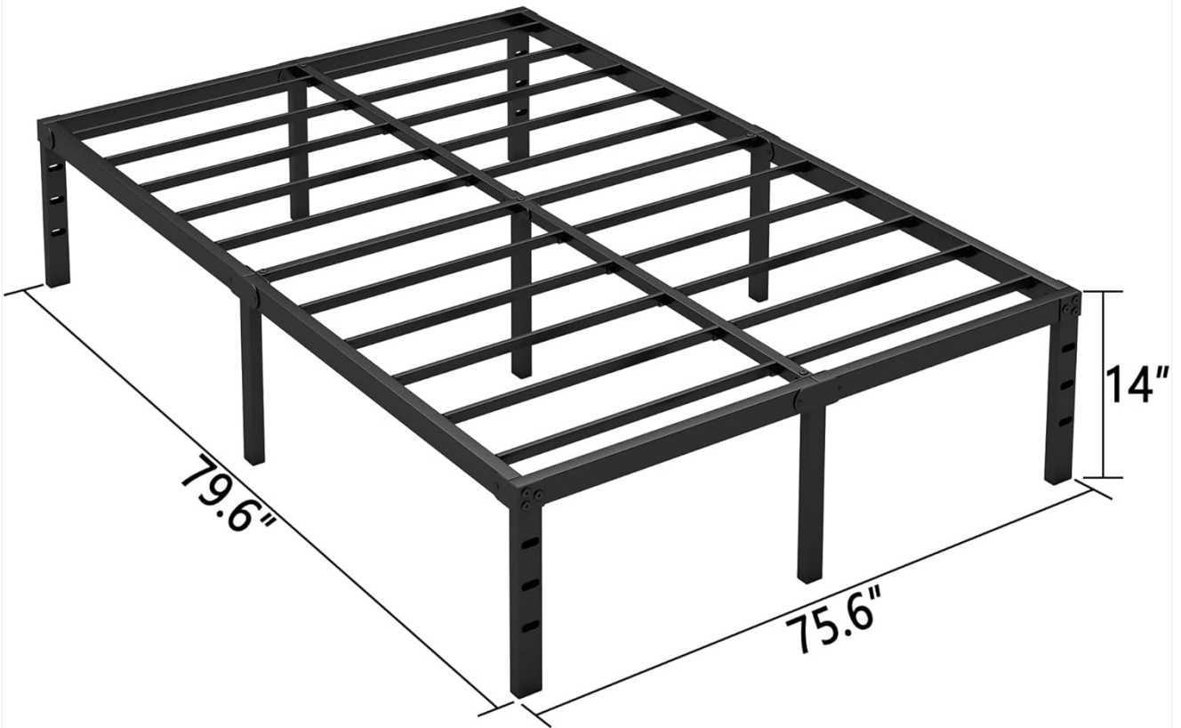
Image: Dimensional diagram of the Hafenpo King Bed Frame.
