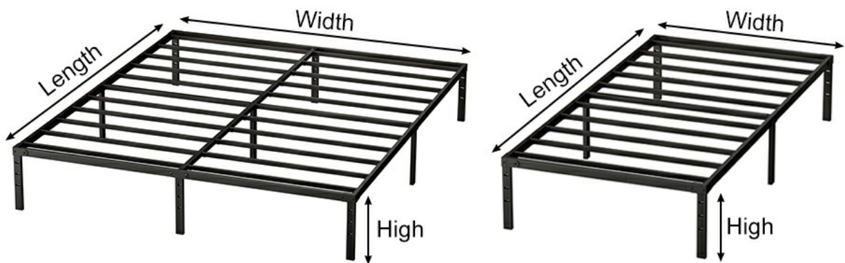
Image: Dimensional diagram of the Hafenpo King Bed Frame.
