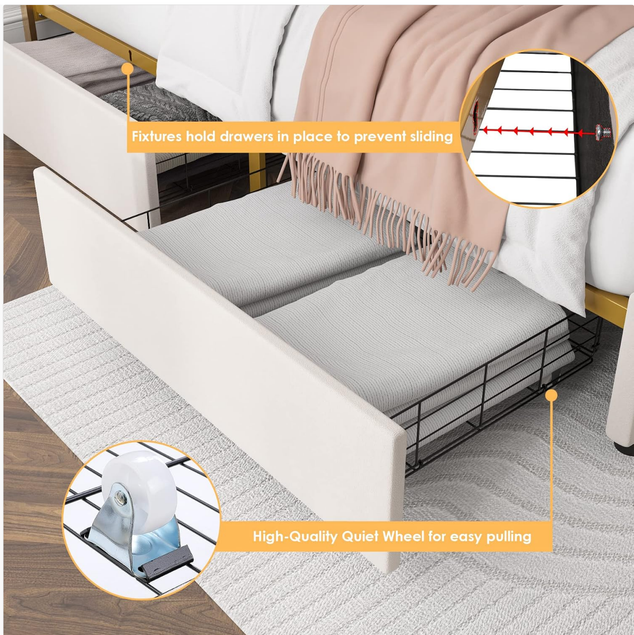
Figure 3: Detailed view of the storage drawer mechanism, illustrating the smooth-gliding wheels and secure locking fixtures.
