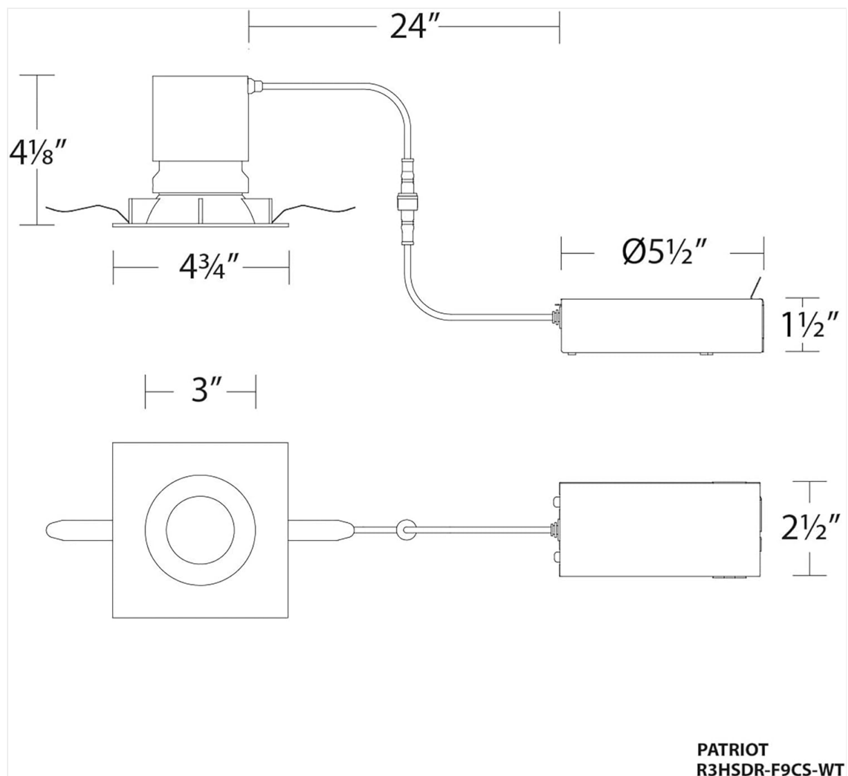
Figure 4: Dimensional drawing with measurements for installation.
