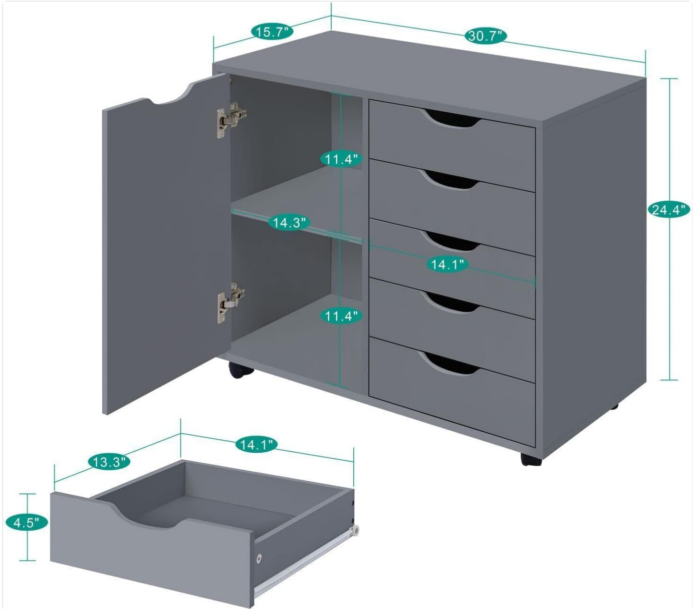
Image: Detailed dimensions of the cabinet, including internal shelf and drawer measurements, useful for assembly and planning.
