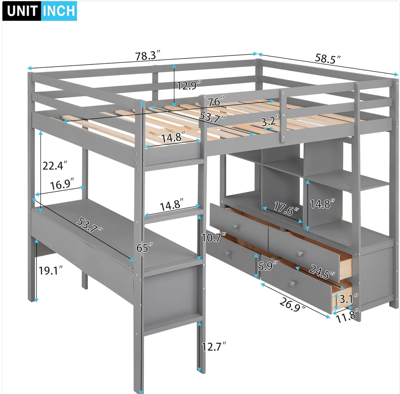
Image 8.1: Dimensional diagram of the Merax Full Size Loft Bed.
