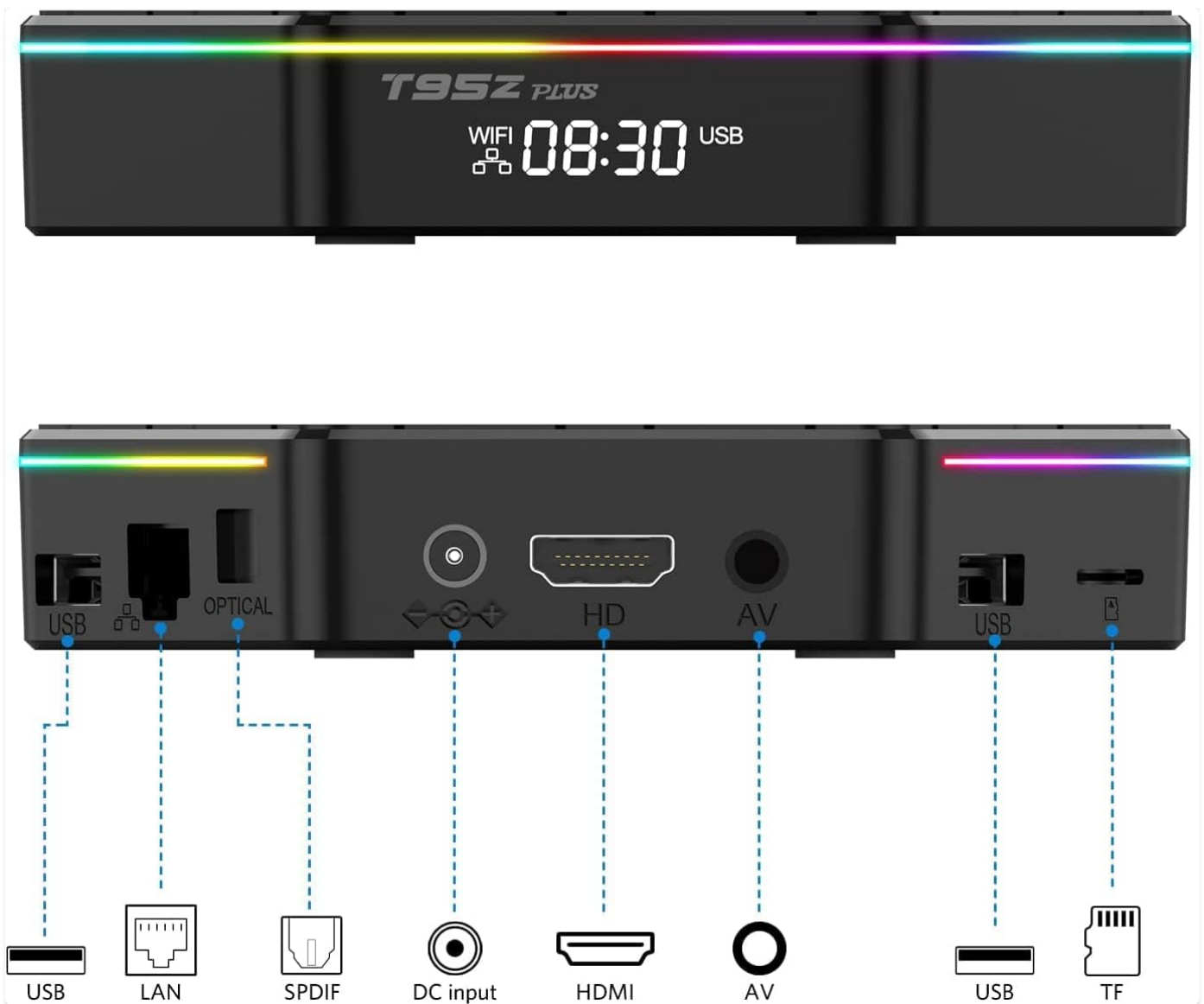
Image: Detailed view of the TV box ports, including USB, LAN (Ethernet), SPDIF (Optical), DC input for power, HDMI, AV, and TF card slot.
