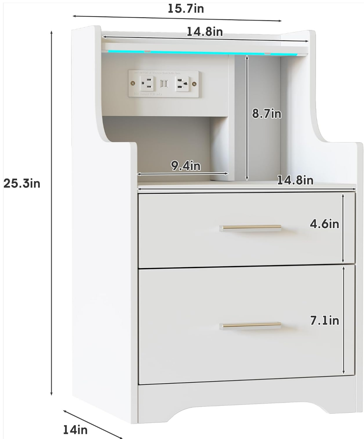
Figure 5: Product Dimensions
