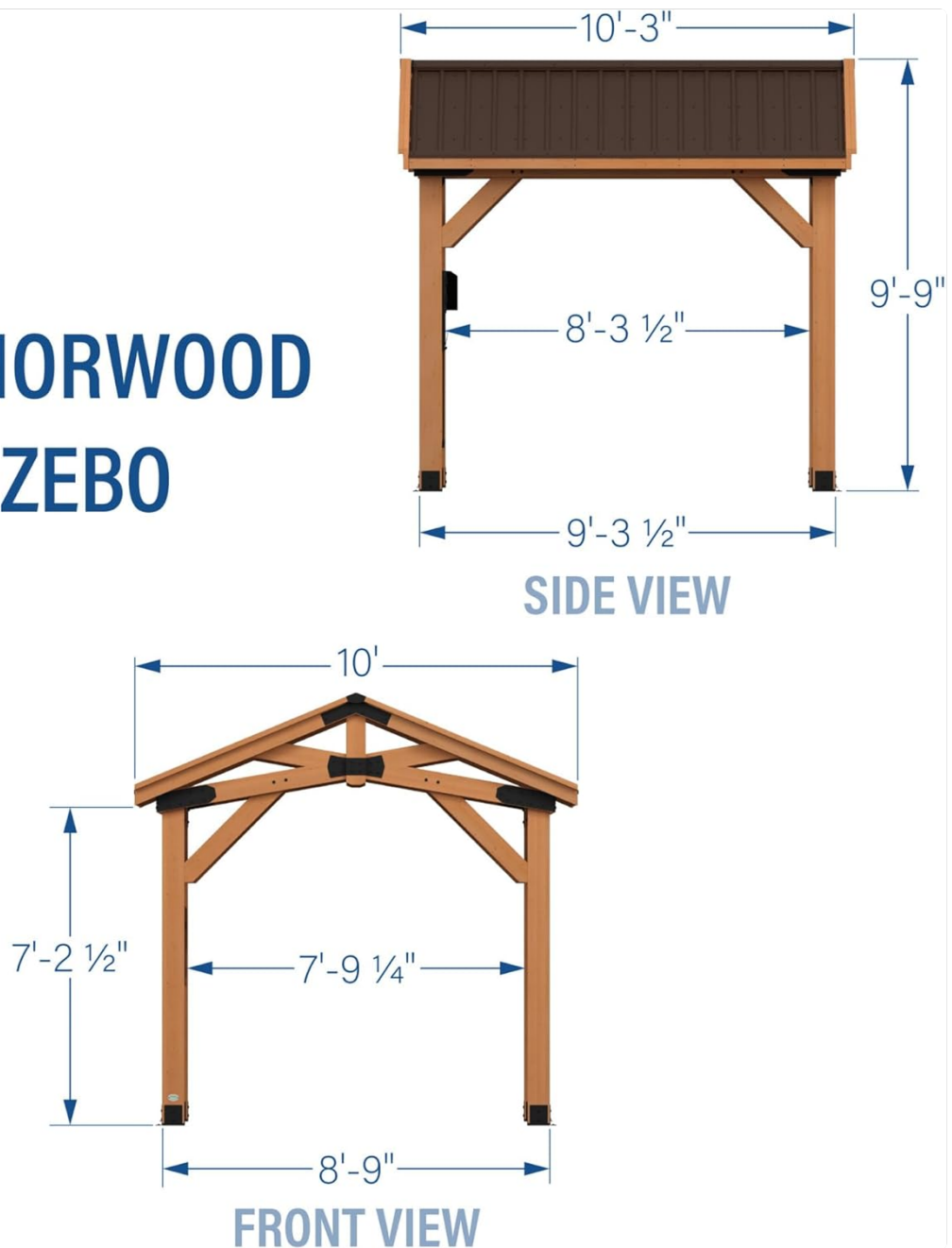
Figure 5: Detailed dimensions for the Norwood 10' x 10' Gazebo.
