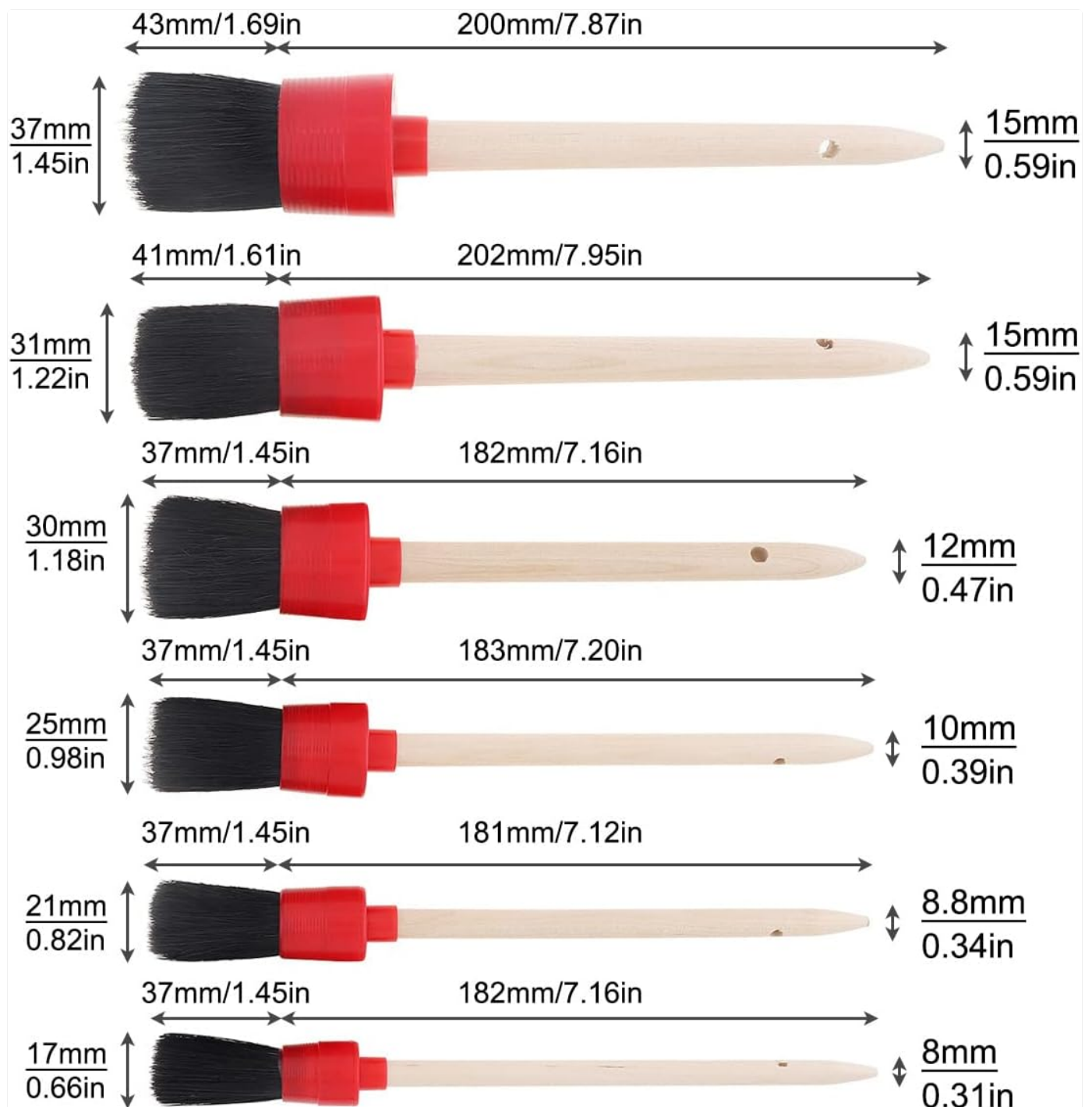
Figure 3.1: Detailed dimensions for each of the 6 auto detailing brushes, showing varying lengths and brush head diameters.
