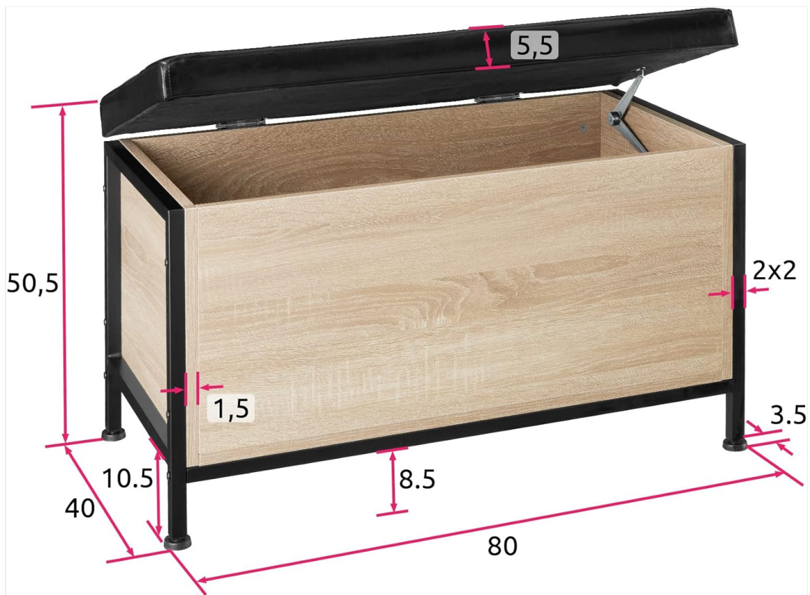
Image: Dimensional diagram of the storage box, illustrating overall and internal measurements.
