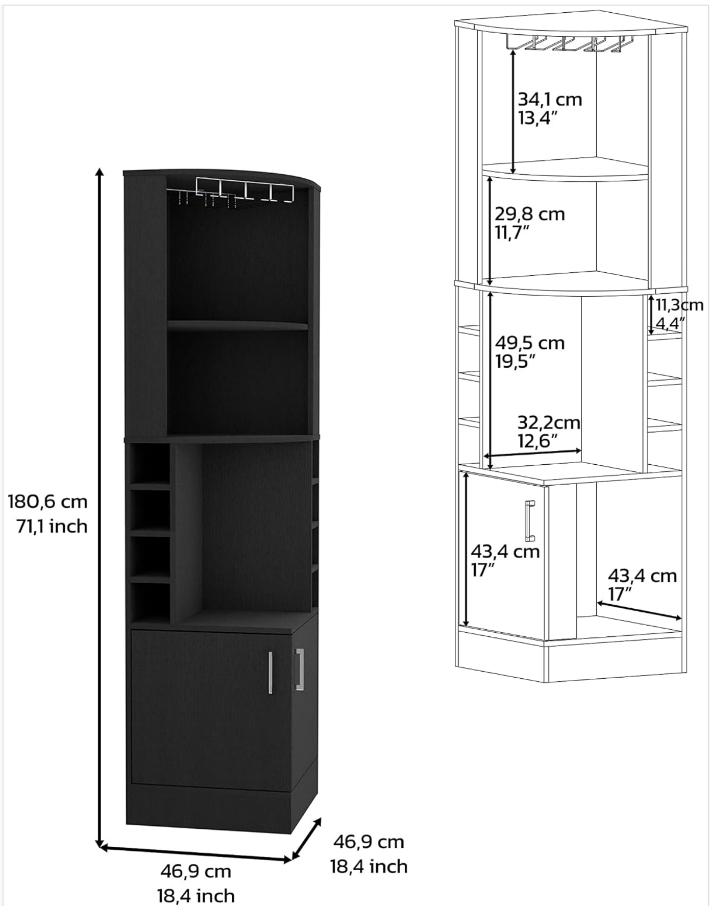
Image: Detailed dimensional diagram of the Cairo Corner Bar Cabinet, showing height, width, and depth measurements for various sections.
