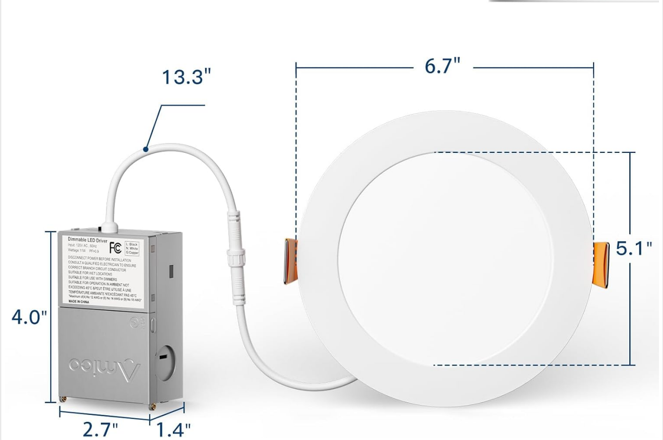
Image 2: Technical drawing providing the dimensions of the Amico 6-inch recessed light and its associated junction box, including the advised hole cutout size of 6.25 inches.
