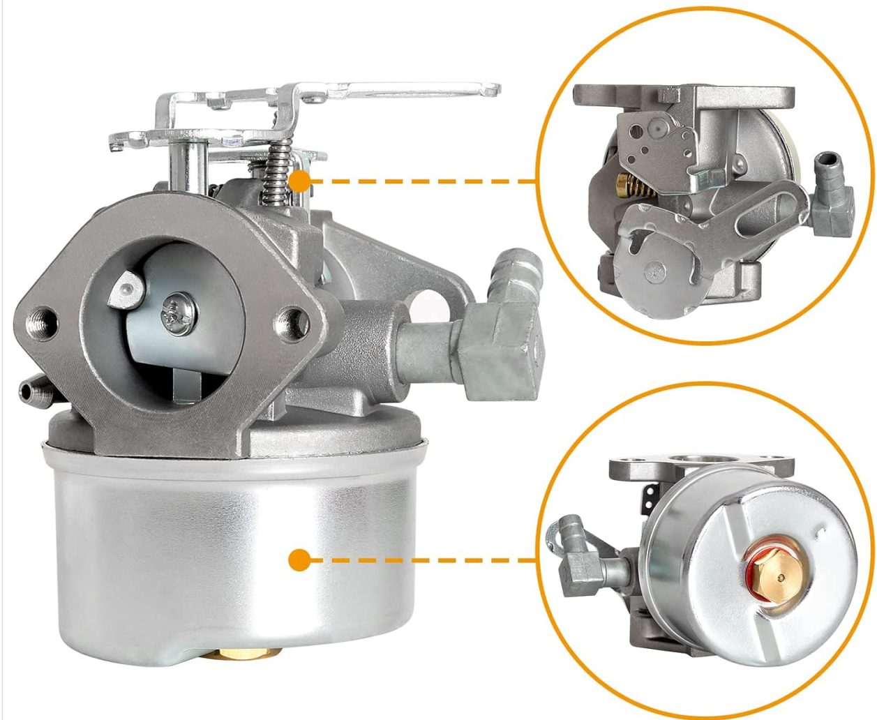
Image: Detailed views of the CLSR2U 640084B Carburetor, highlighting its various ports and adjustment points.
