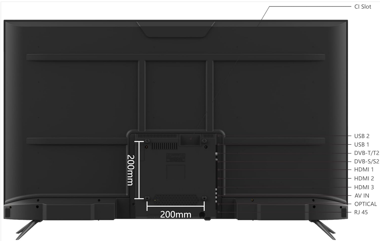
Figure 3.2: Rear panel of the SMART TECH 55-inch TV, displaying the available connection ports. These include USB 1, USB 2, DVB-T/T2 (Antenna), DVB-S/S2 (Satellite), HDMI 1, HDMI 2, HDMI 3, AV IN, Optical Audio Out, and RJ45 (Ethernet) port. A CI Slot is also visible.
