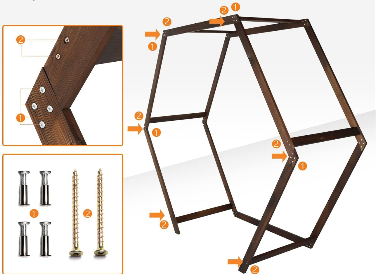
Figure 3.1: Detailed assembly diagram illustrating the connection points and hardware for the arbor.
