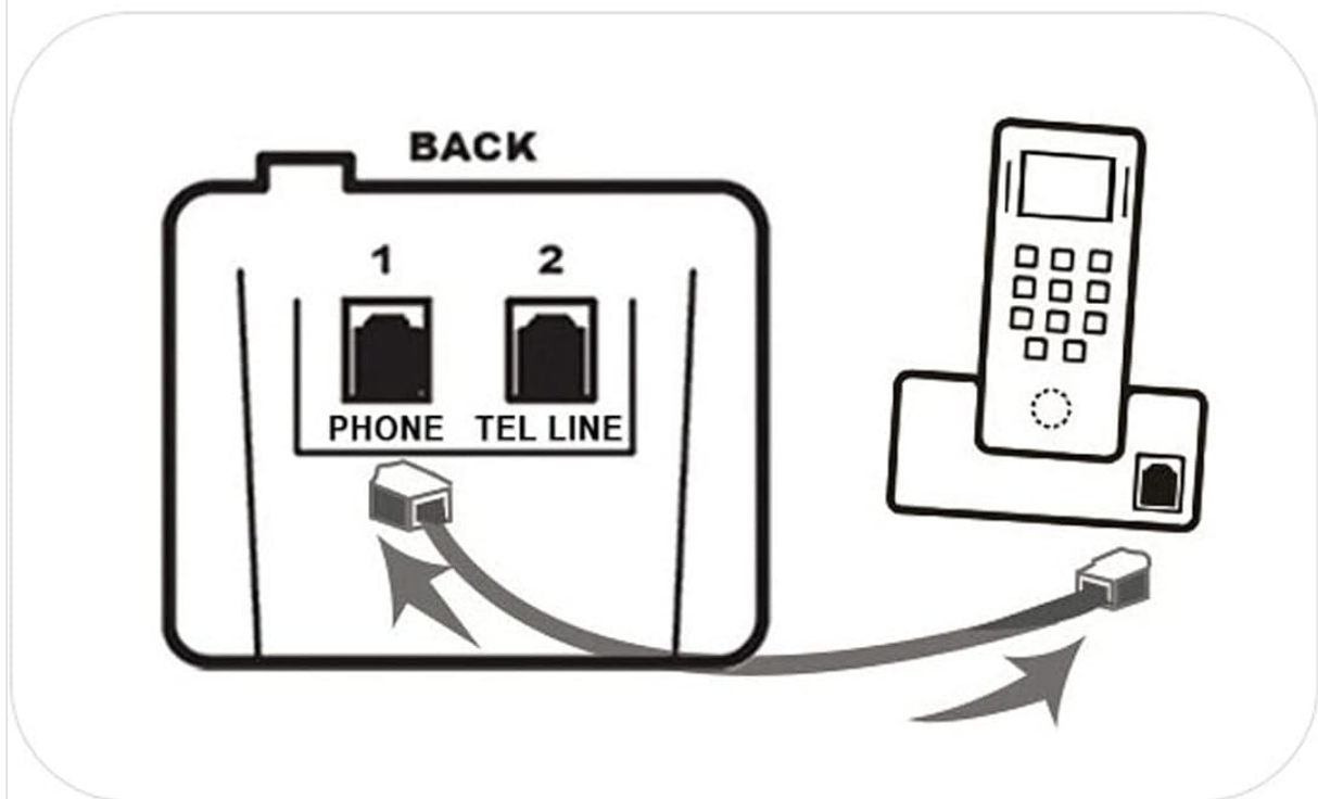
Image: Rear view of the call blocker showing the 'PHONE' and 'TEL LINE' ports, along with a diagram illustrating how to connect the device between the telephone wall jack and your landline phone.
