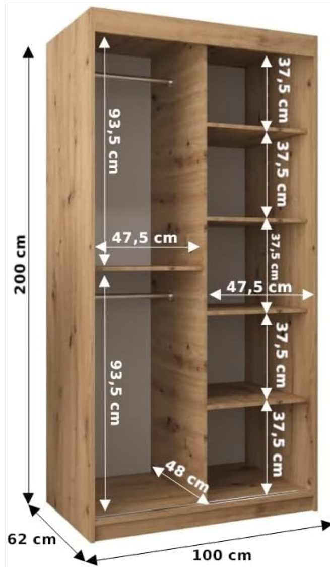
Image 7.1: Dimensional diagram of the wardrobe.
