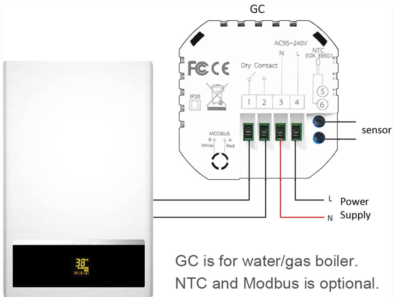
Image: Wiring diagram for the Haofy BHT 8000GB thermostat, illustrating connections for power supply, load (boiler), and optional NTC sensor and Modbus.
