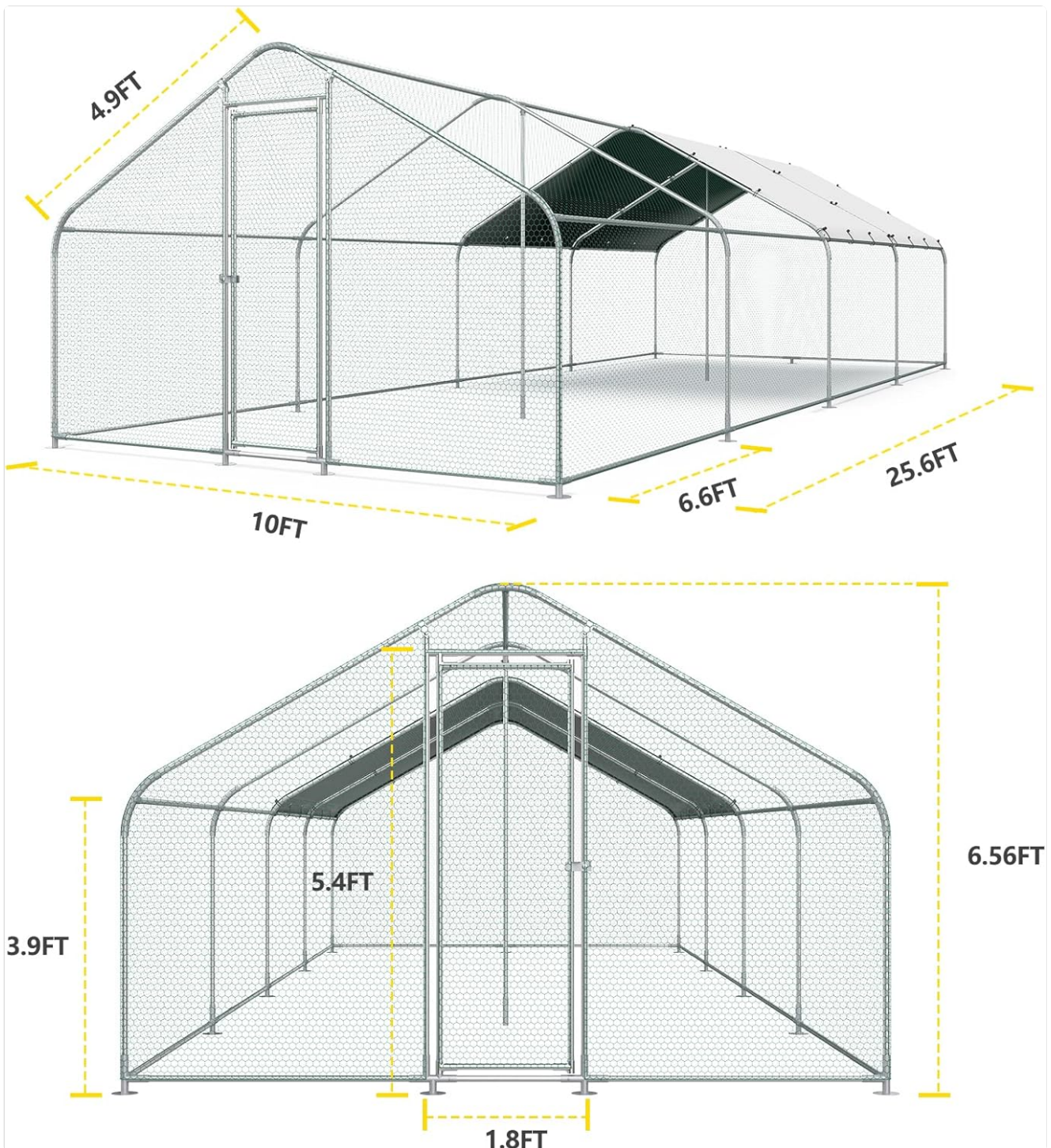
Image: A detailed diagram illustrating the overall dimensions of the chicken coop, including length, width, and height measurements for various sections.
