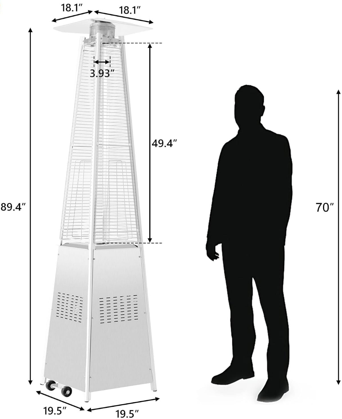
Image 8.1 : Product dimensions.
