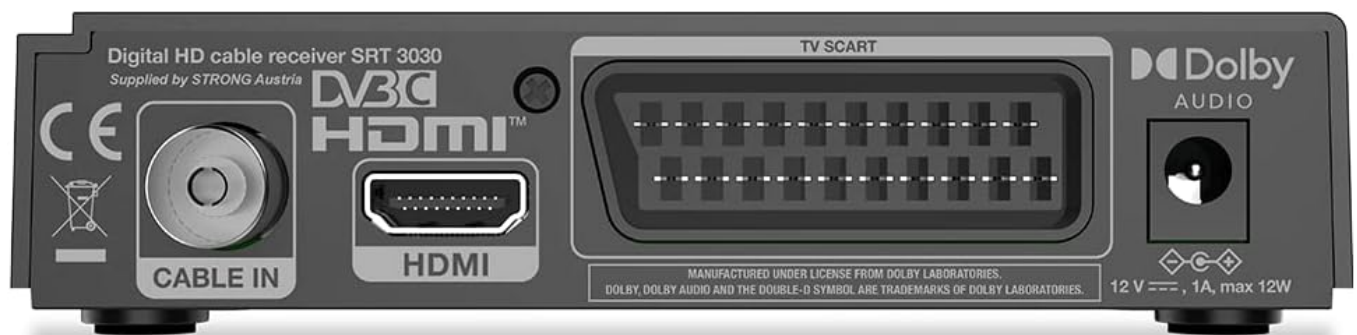
Figure 3: Rear view of the receiver, showing the "CABLE IN" port, HDMI output, TV SCART connector, and the power input.
