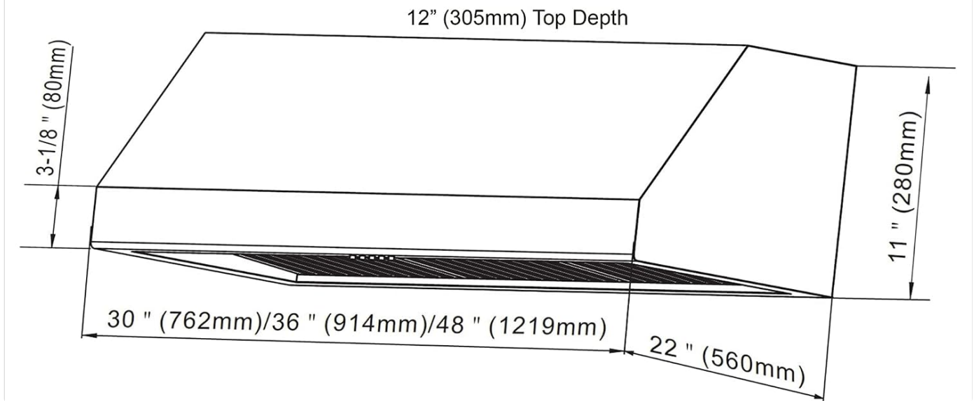
Figure 4: Detailed dimensional drawing of the TRH3606 Range Hood, showing height, width, and depth.
