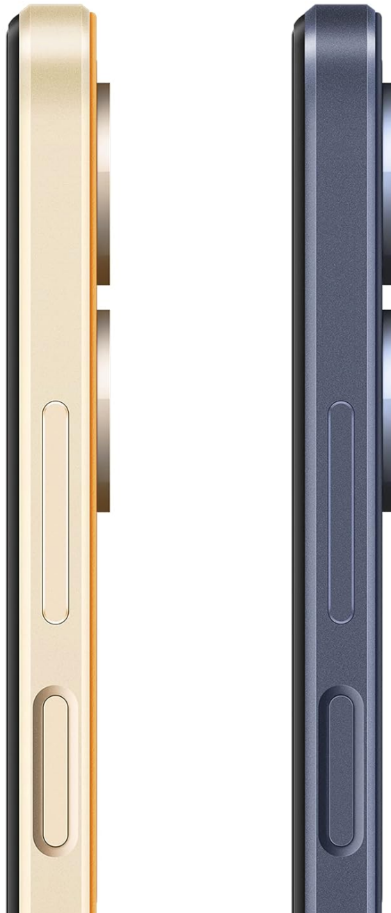
Figure 4: Side view of the OPPO A17, highlighting the fingerprint sensor.
