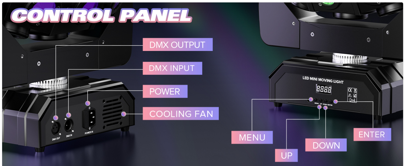
Figure 3.1: Detailed view of the control panel buttons and rear connection ports including DMX In/Out and Power In/Out.
