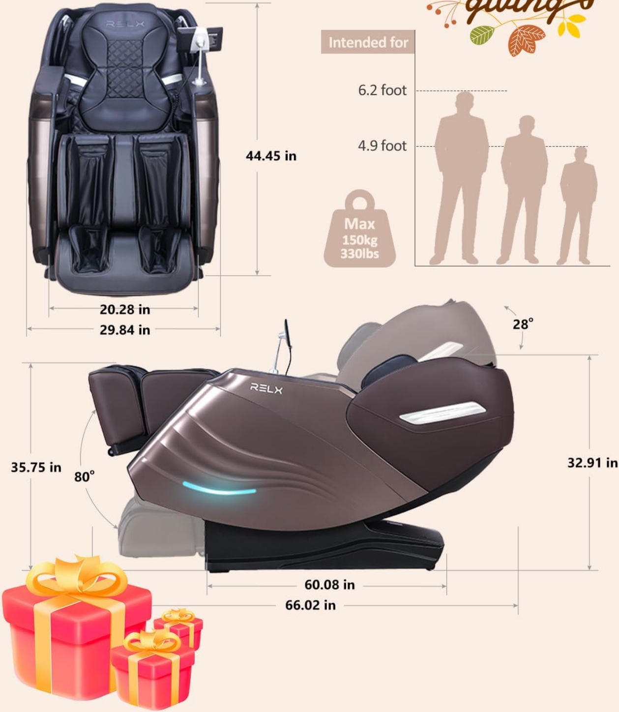
Figure 15: Product Dimensions and User Recommendations
