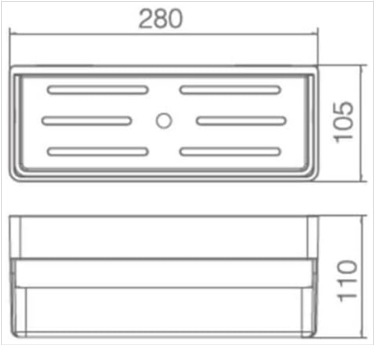
Figure 2: Technical drawing showing the dimensions of the IMEX Rectangular PVC Soap Dish. The top view indicates a length of 280mm and a width of 105mm. The side view shows a total height of 110mm.
