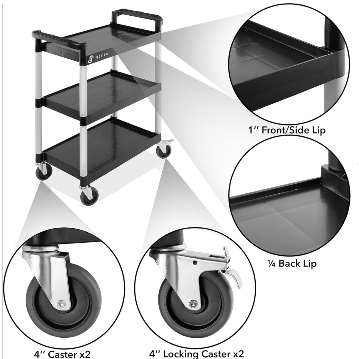
Image 4.1: Detail of shelf lip (1-inch front/side, 1/4-inch back) and 4-inch casters (swivel and locking).
