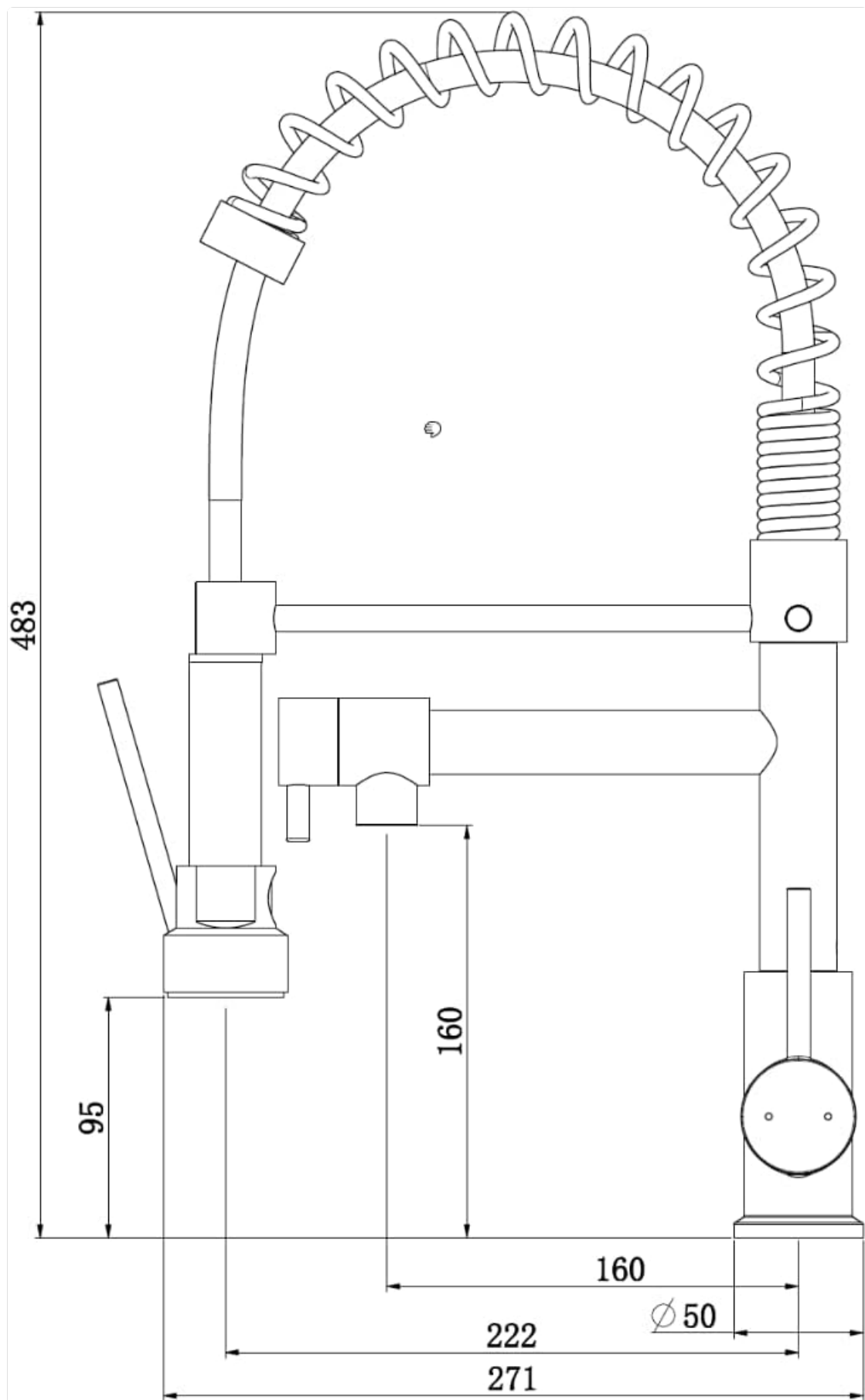
Image: Technical drawing illustrating the dimensions of the ESSEBAGNO Big Pro 9019781 faucet, including height, width, and spout reach.
