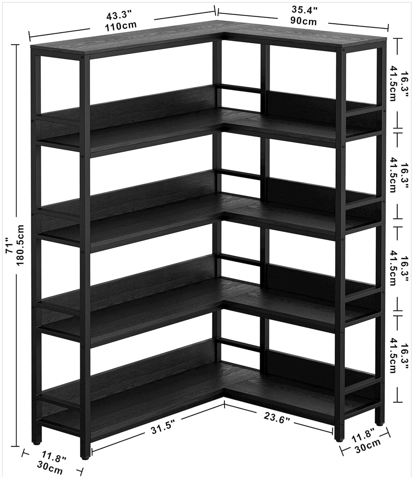
Image: Detailed dimensions of the IRONCK 5-Tier Industrial L-Shaped Corner Bookshelf, showing height, width, and depth measurements for both sides of the L-shape.
