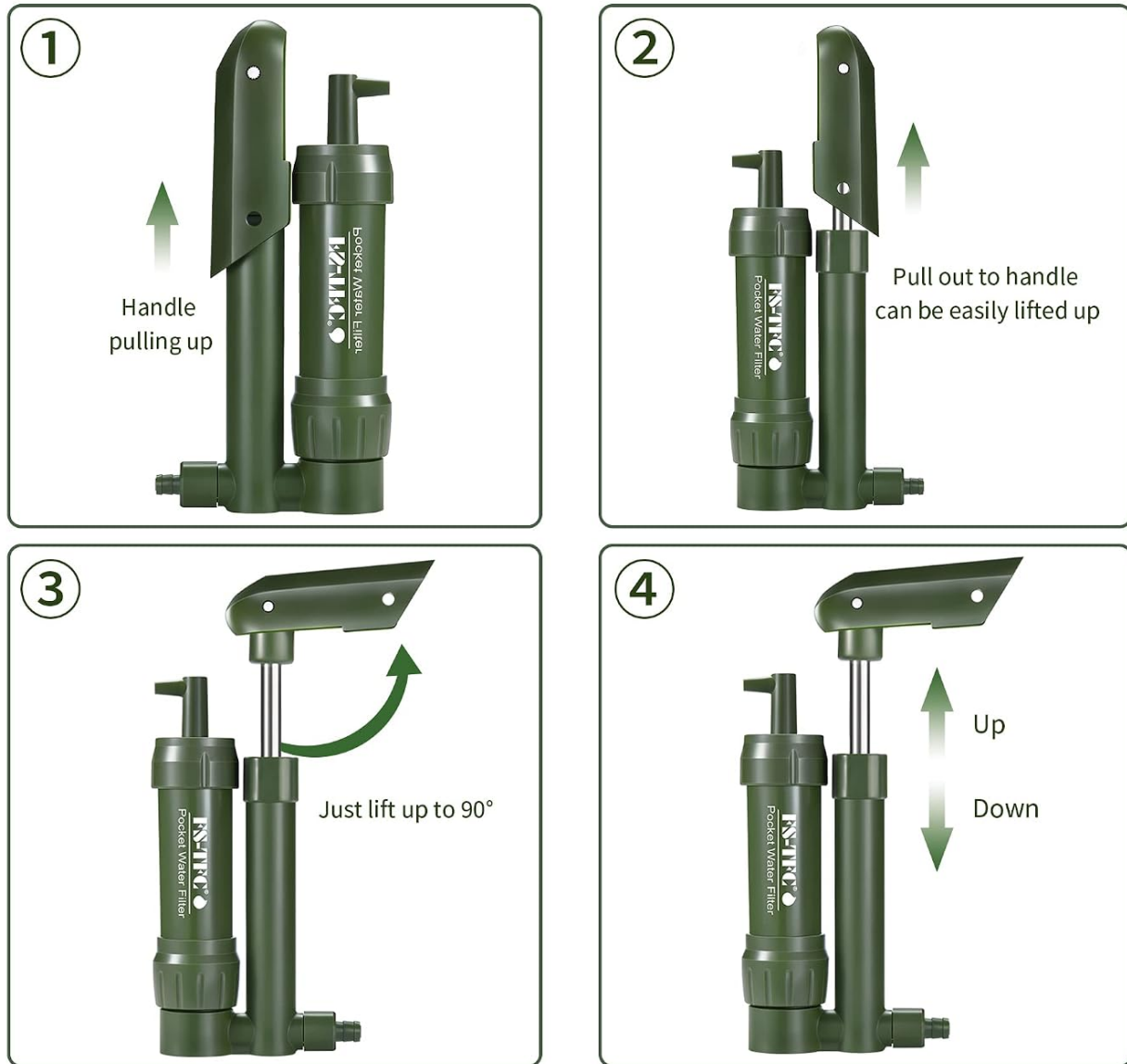
Figure 5: Folding Handle Operation.
