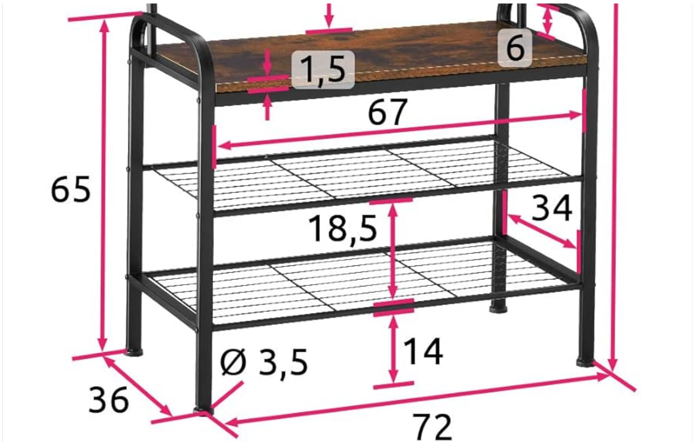
Figure 2: Dimensions diagram for assembly reference.
