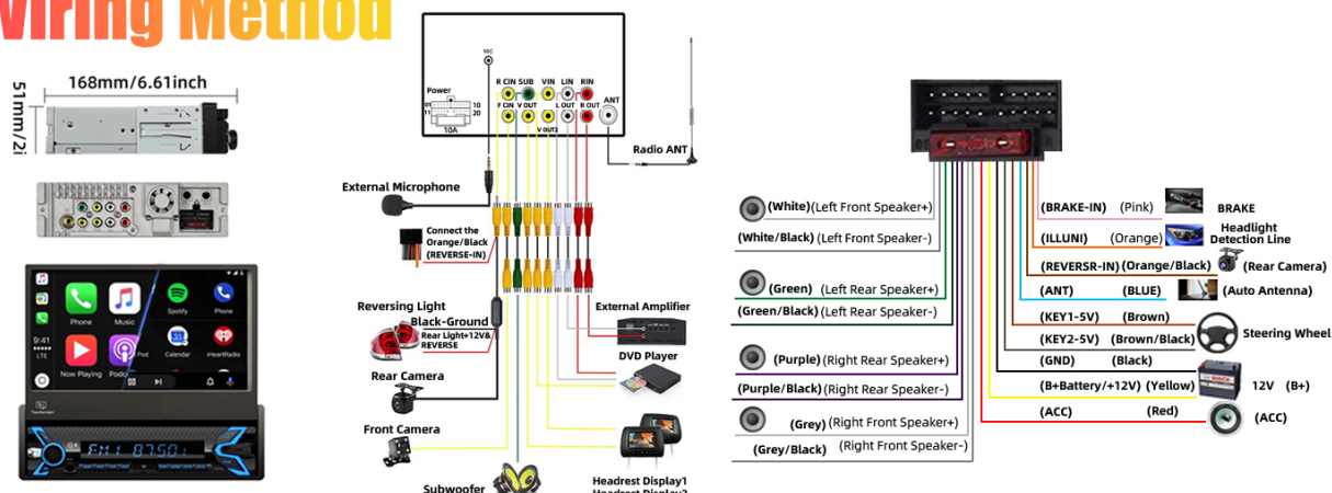
Figure 4.1: Wiring Method for the Car Stereo.
