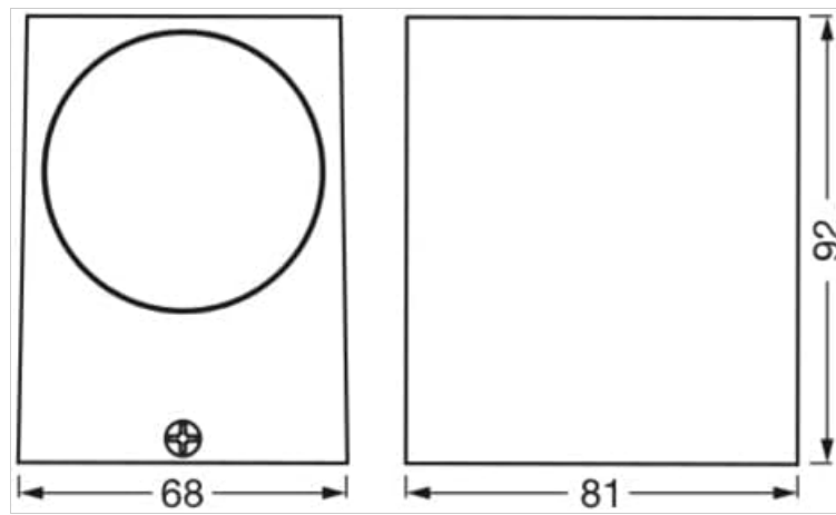
Image 4.1: Technical diagram illustrating the dimensions of the LEDVANCE ENDURA Classic Square Down light. The front view shows a width of 68mm, and the side view shows a depth of 81mm and a height of 92mm. These measurements are crucial for planning installation.
