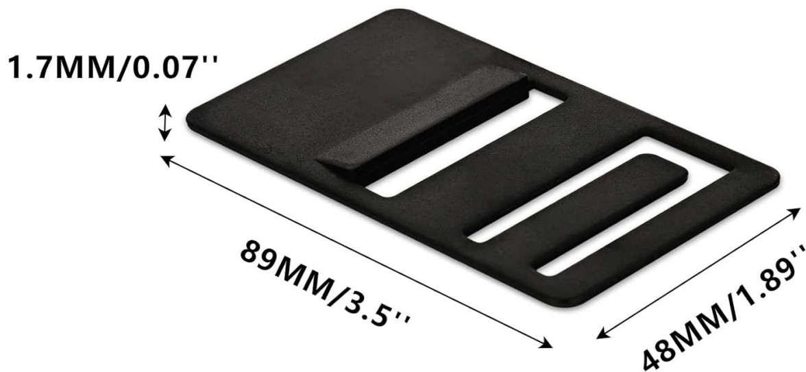
Image 6.1: A detailed size map of the Carkio RV Refrigerator Airing Device, showing its dimensions: 89mm (3.5 inches) in length, 48mm (1.89 inches) in width, and 1.7mm (0.07 inches) in thickness.
