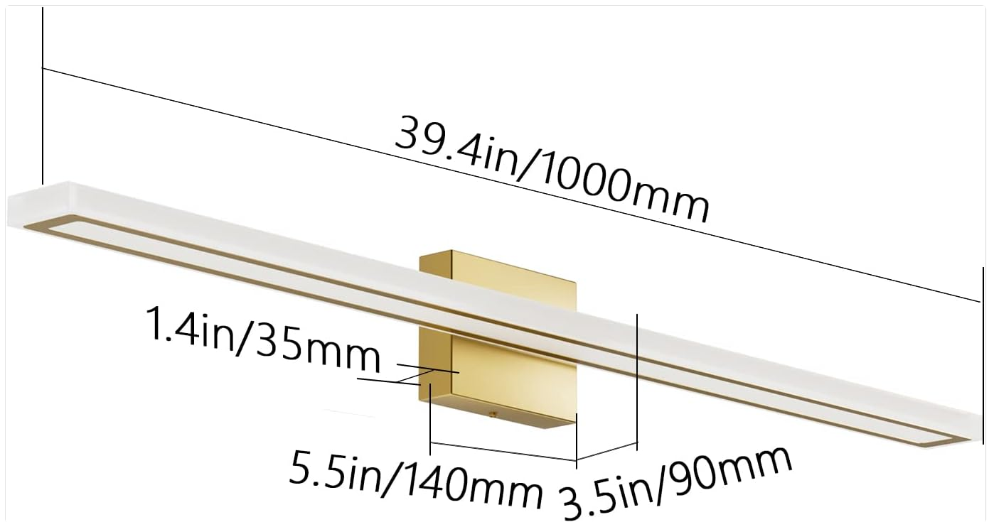
Figure 1: Product Dimensions. This image displays the key dimensions of the Ralbay 40-inch LED Vanity Light Fixture, including its overall length of 39.4 inches (1000mm), depth from the wall, and the size of the mounting base.
