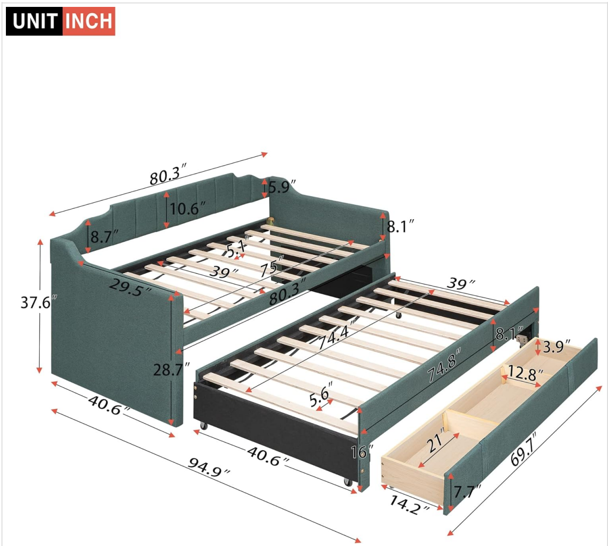
Image 4.1: Exploded view with dimensions for assembly.
