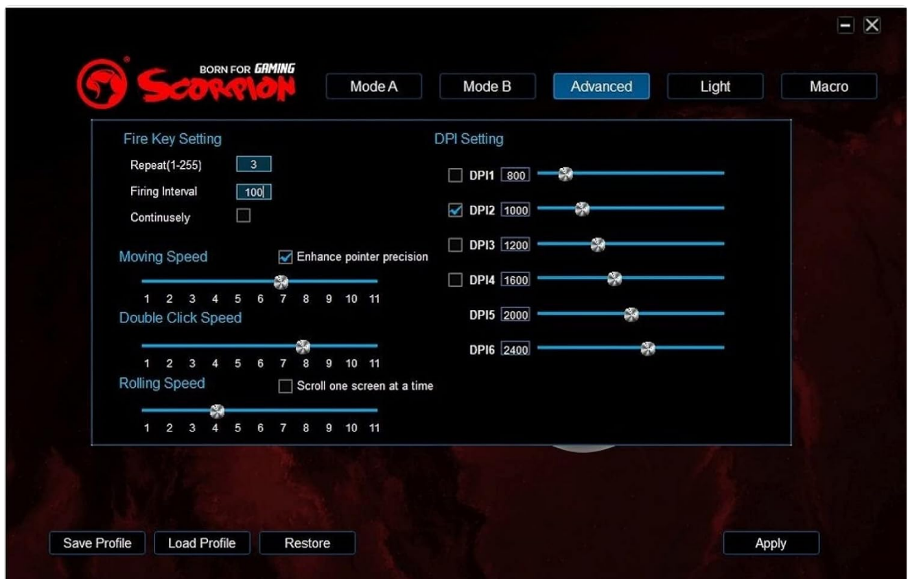
Figure 7: Screenshot of the Marvo gaming mouse software's advanced settings, including Fire Key Setting, DPI Setting (800-2400), Moving Speed, Double Click Speed, and Rolling Speed adjustments.
