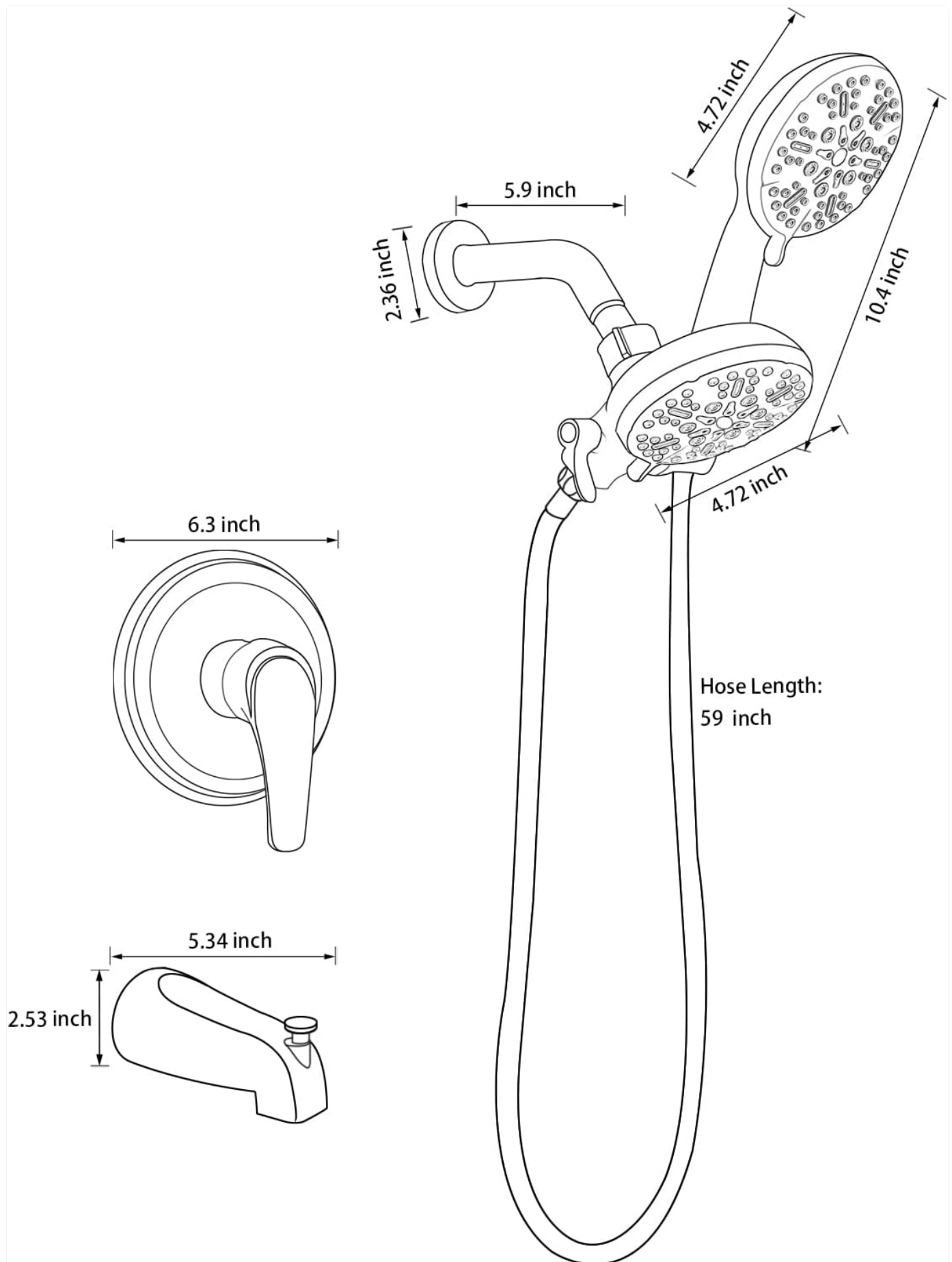
Image: Dimensional drawing of the DIFEINI Bathtub and Shower Faucet Set components.
